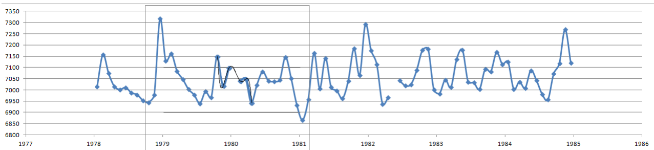
Figure 44 - Subset of the monthly sea level in Brest. The black line is the polynomial interpolation used to fill a short period gap.
