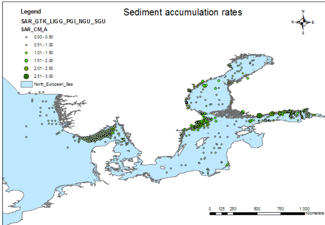
Figure 4. Sediment accumulation rates (cm/year) in the Baltic Sea/Greater North Sea.
