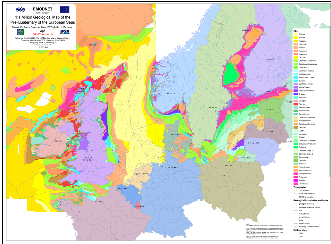
Figure 5. Sea-bed geology at 1:1 million scale.
