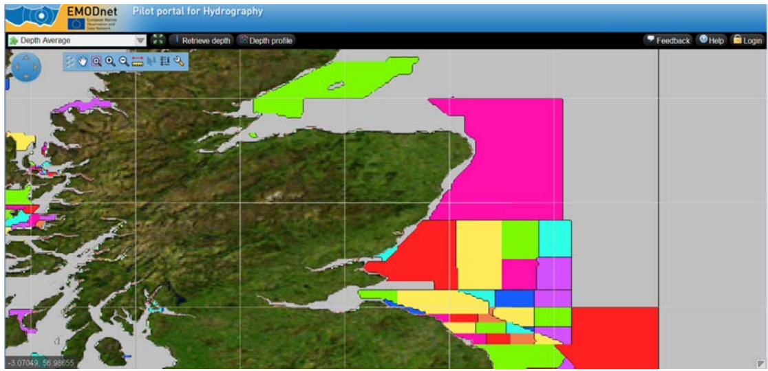
Image: resulting DTM near UK - sources layer indicating surveys and GEBCO (= grey)
