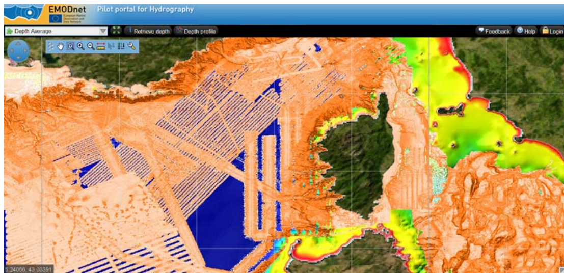
Image: resulting DTM near Corsica with standard deviation per DTM gridcell
