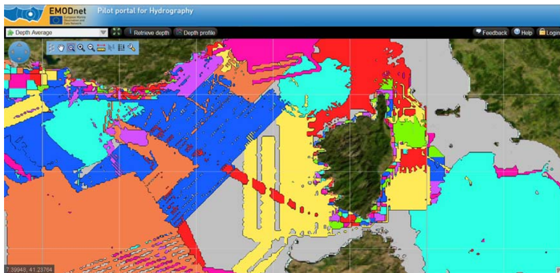
Image: resulting DTM near Corsica - sources layer indicating surveys, composite DTMs and GEBCO (= grey)
