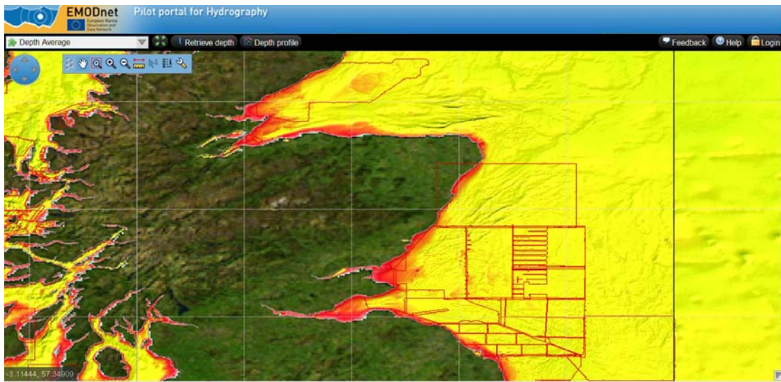
Image: resulting DTM near UK with tracks of the surveys as indicated by the CDI metadata records
