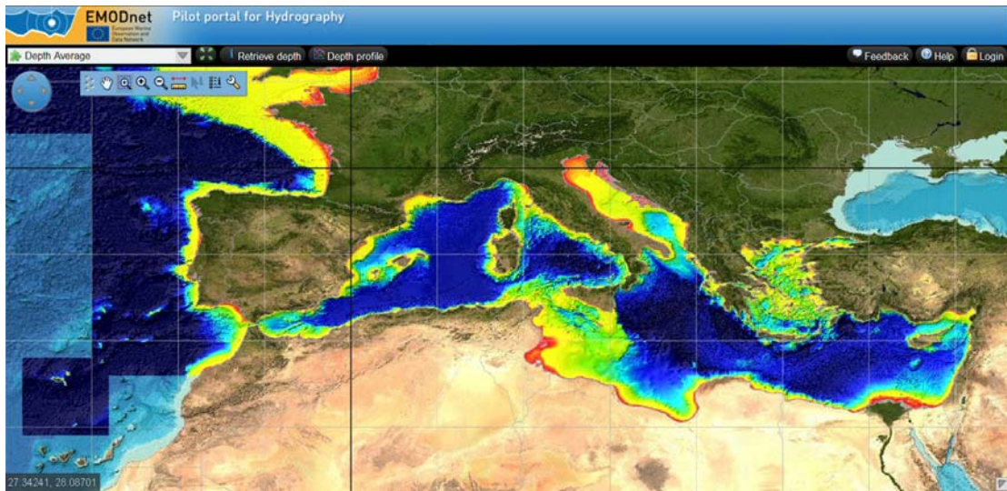
Image: New DTM for Western and Central Mediterranean Sea
